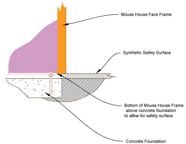
Cross Section of recommended Safety surface Treatment
