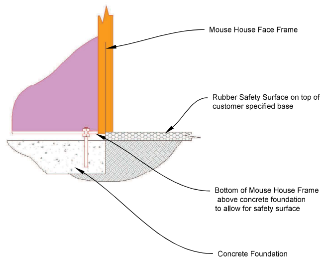
Cross Section of recommended Safety surface Treatment
